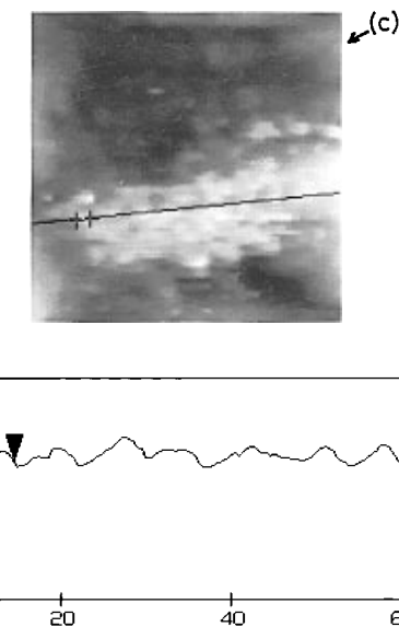
Figure 7. (a) TEM image of thiol-derivatized Pt nanoparticles prepared by \text{NaBH}_4 reduction. (b) The histogram shows the particle size distribution (mean diameter = 4.1 nm). (c) STM image of a crystallite formed by spherical Pt nanoparticles. (d) The line profile of the crystallite in c with the two arrows marking the diameter of the particle.
